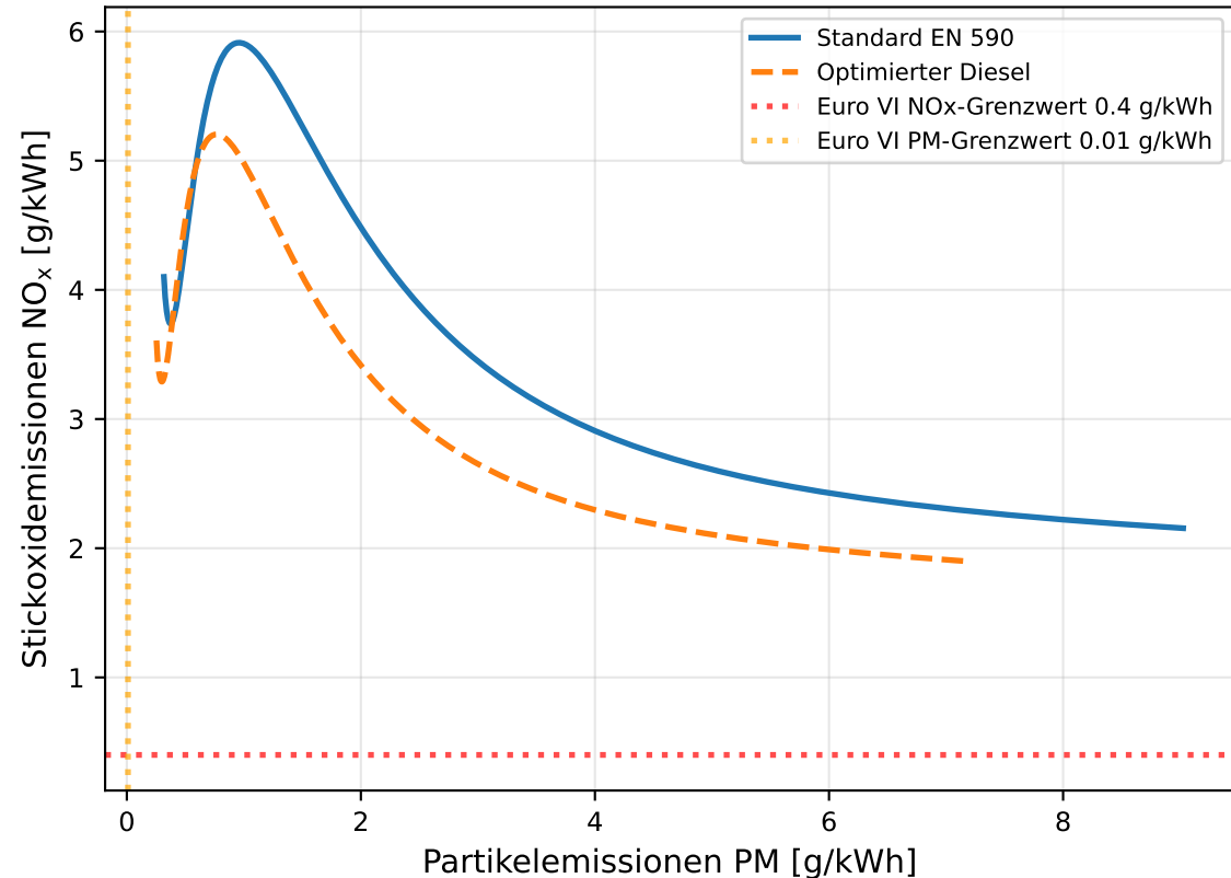
NO x -PM-Tradeoff
