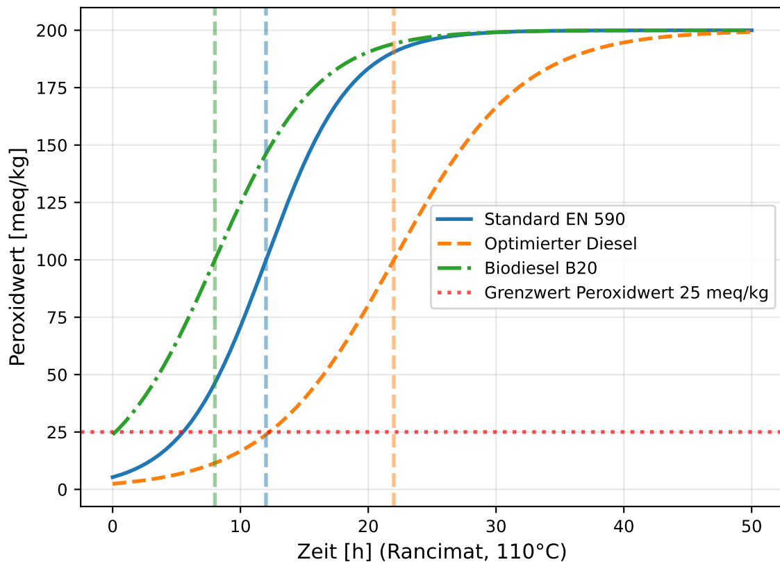
Oxidationsstabilitaet (Rancimat-Test)
