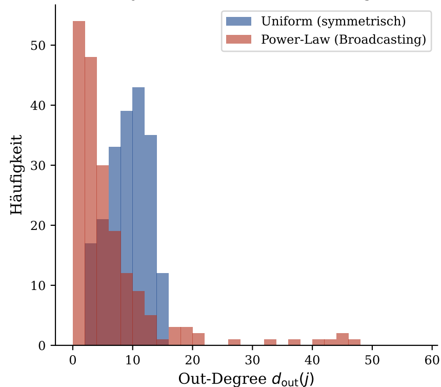
Out-Degree-Verteilung: Symmetrisch vs. Broadcasting
