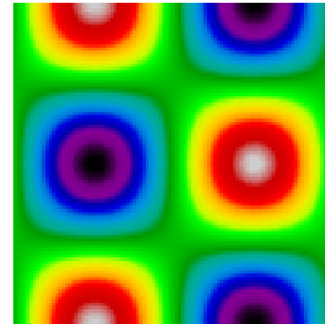
nipy_spectral
