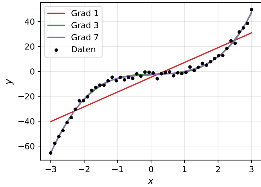
Polynominterpolation (NumPy)
