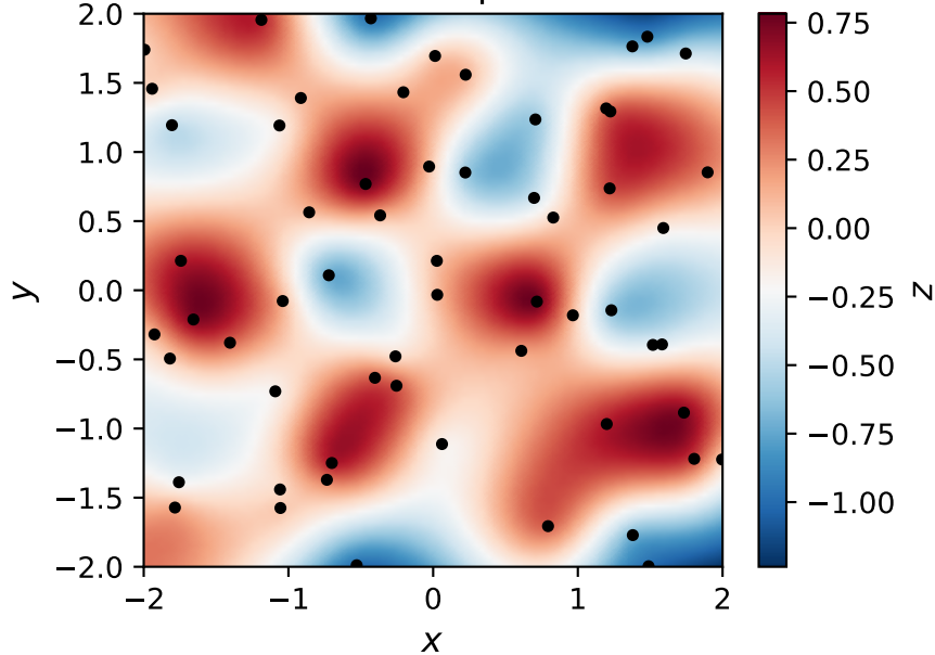
RBF 2D-Interpolation
