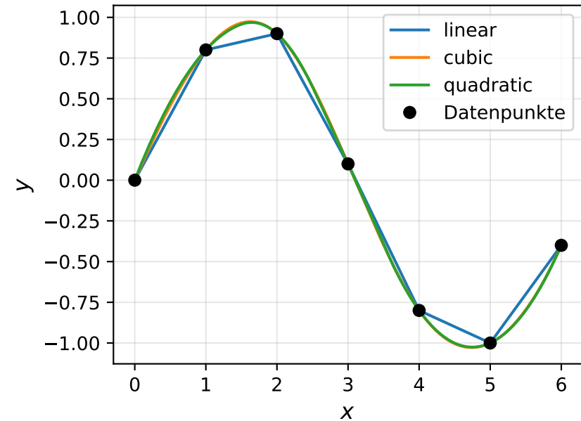
Spline-Interpolation (SciPy)
