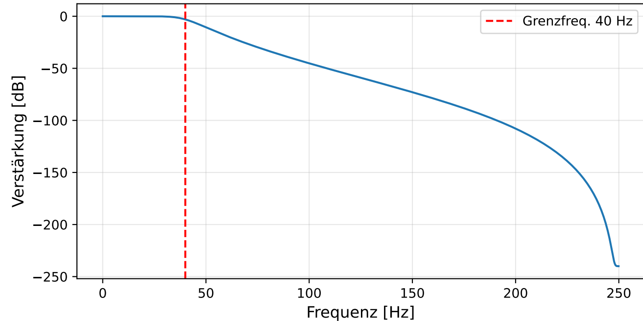
Frequenzgang Butterworth-Filter
