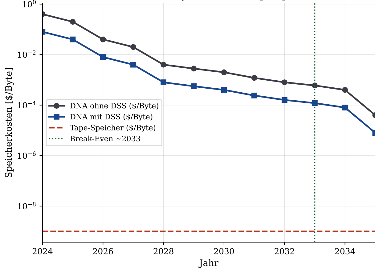
Break-Even-Analyse: DNA vs. Tape-Speicher
