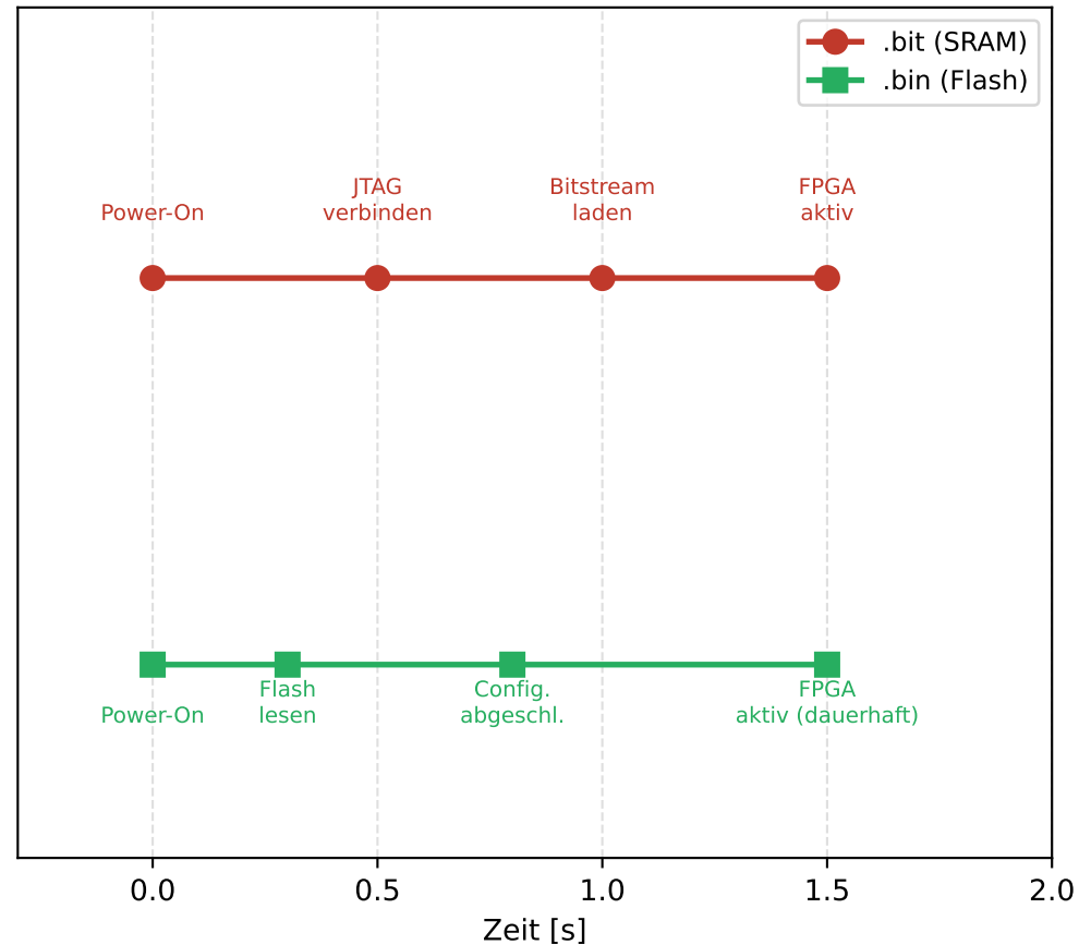
Boot-Sequenz: SRAM vs. Flash
