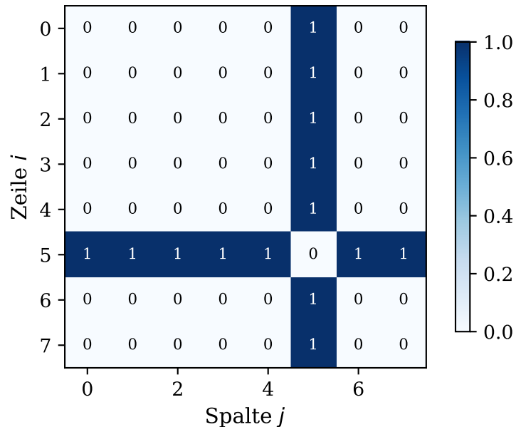
Adjazenzmatrix A_{G_f} (Ziel-Subgraph \omega = 5 )
