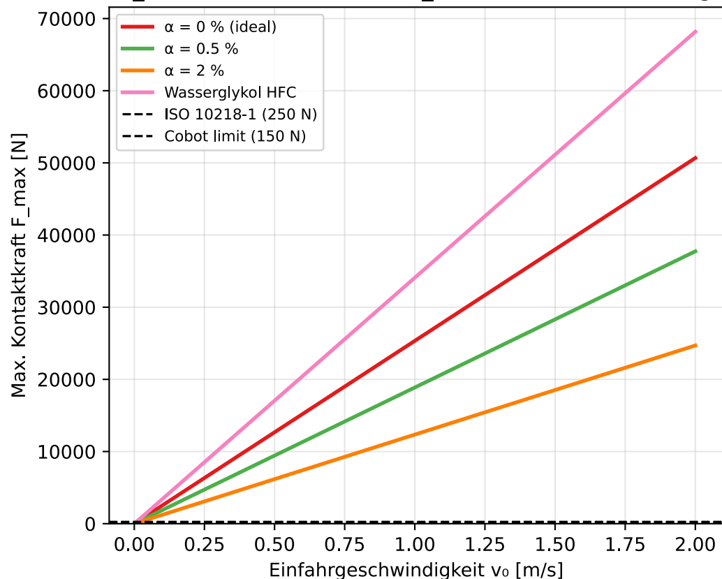
F_{max}(v_0) - Akkumulator V_{acc} = 0.5 L, m = 50.0 kg
