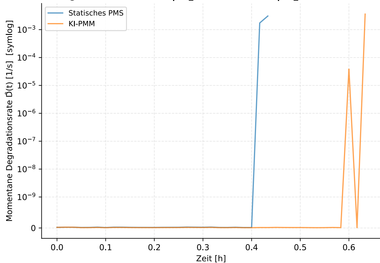
Degradationsrate LP2 | \hat{D}_{stat} = 1.78e-04 | \hat{D}_{AI} = 9.34e-05
