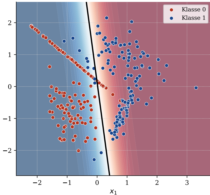
Linear separierbar Accuracy: 92.67%
