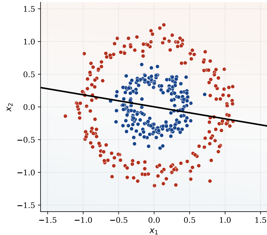
Linear (Grad 1) (Accuracy: 51.00%)
