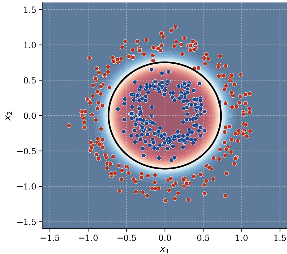
Polynomial Grad 2 (Accuracy: 99.75%)
