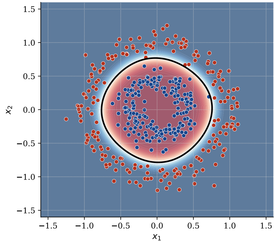
Polynomial Grad 4 (Accuracy: 100.00%)
