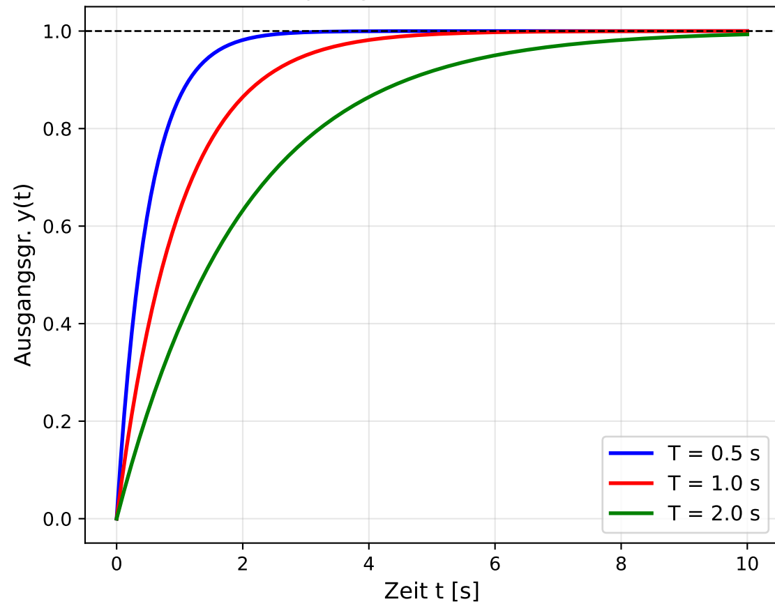
Sprungantwort PT1-Glied
