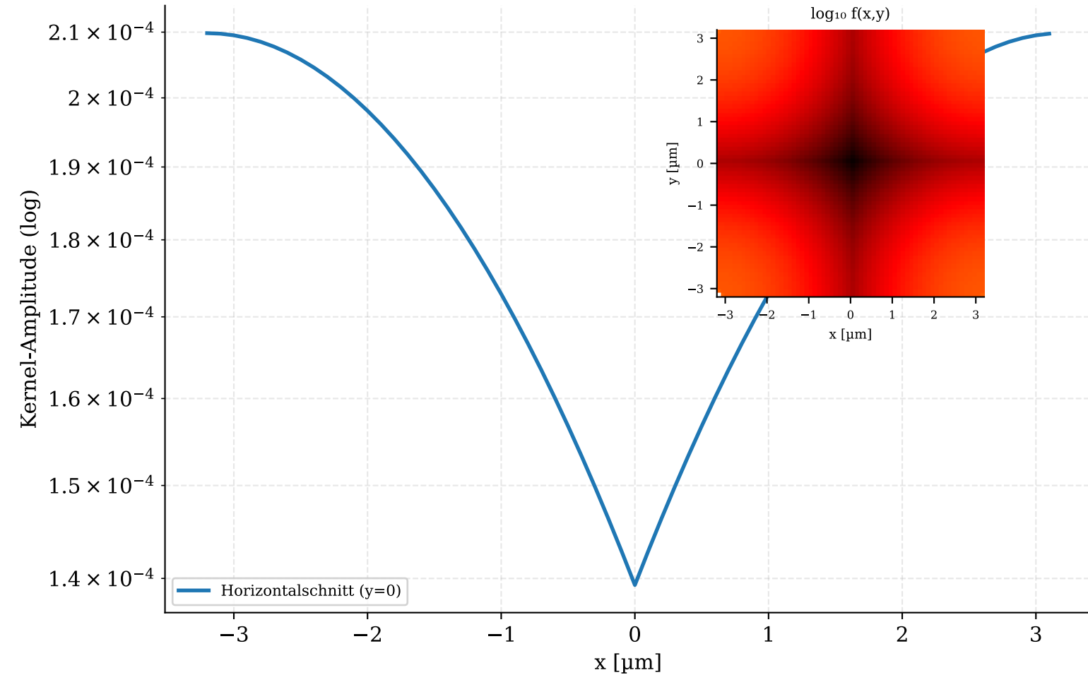
2D-Proximity-Kernel: Schnitt + Heatmap ( N=64 \times 64 , p_x=100 \text{ nm} , \alpha=50 \text{ nm} , \beta=5000 \text{ nm} )
