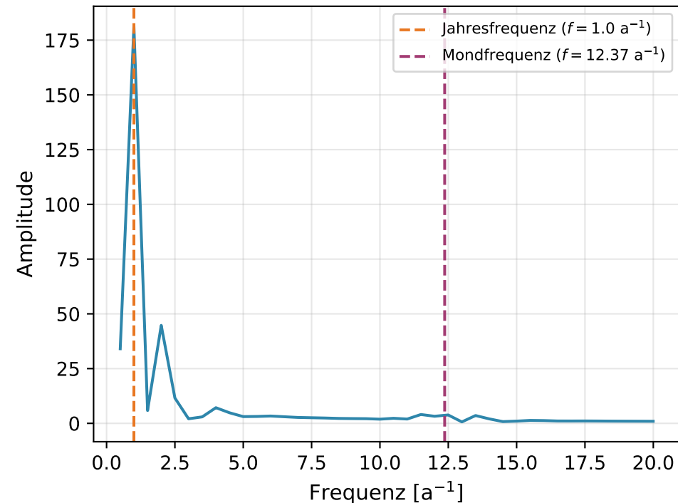
(b) Fourier-Spektrum der Larvenpopulation
