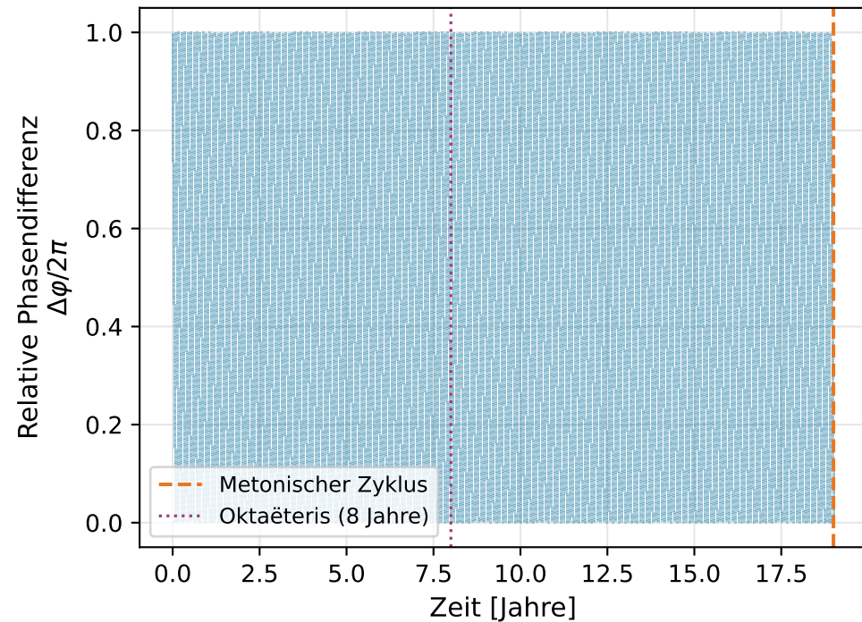
(c) Phasendifferenz Sonne-Mond
