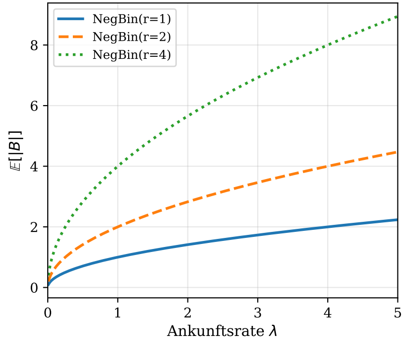
Batchgrösse vs. Last
