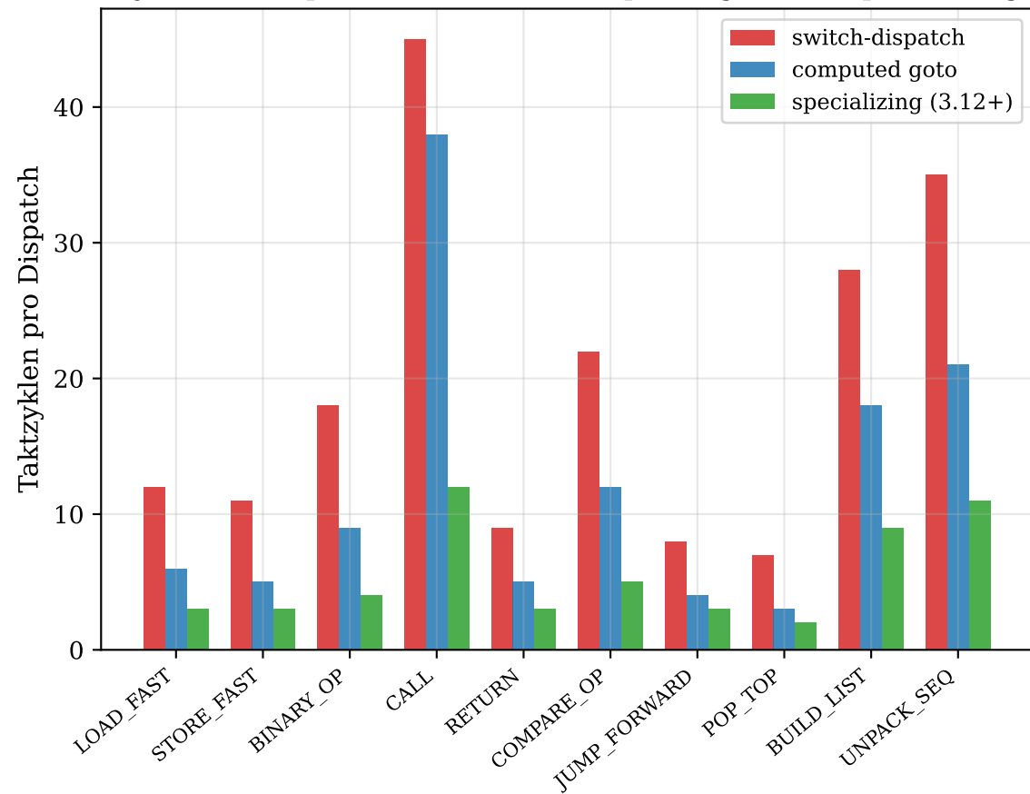
Bytecode-Dispatch: switch vs. computed goto vs. Specializing
