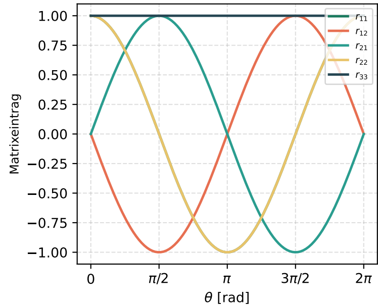
Yaw R_z(\theta)
