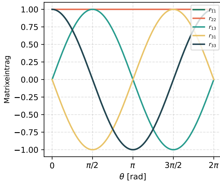
Pitch R_y(\theta)
