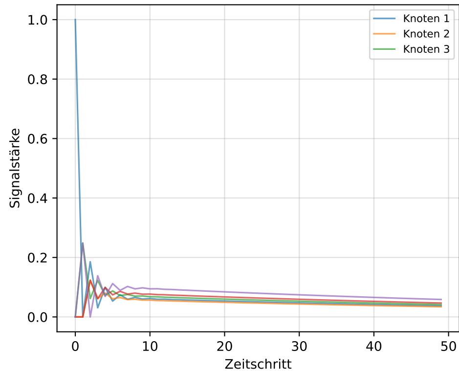
Small-World-Netzwerk \rho(A) = 0.9876
