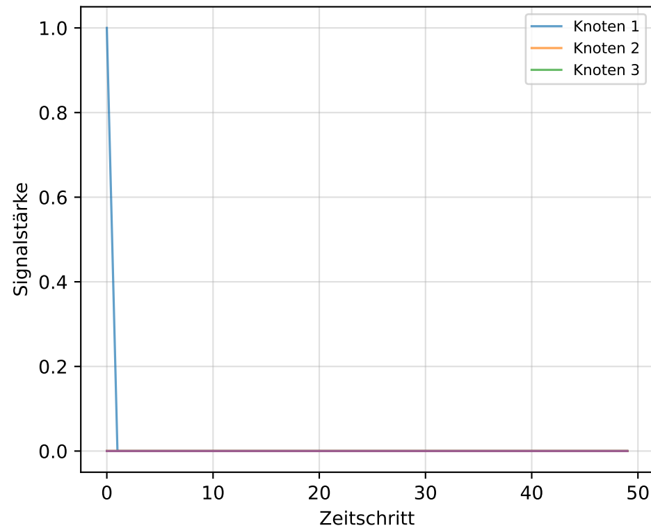
Scale-Free-Netzwerk \rho(A) = 0.9775
