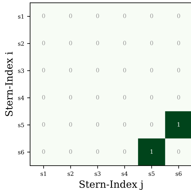
Cluster C (Feldpopulation)
