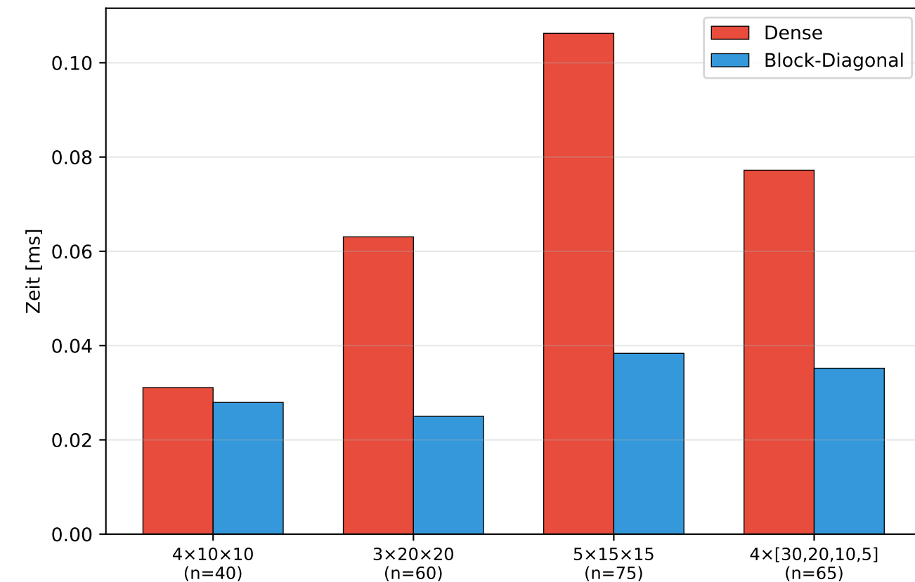
Matrix-Potenz A^5
