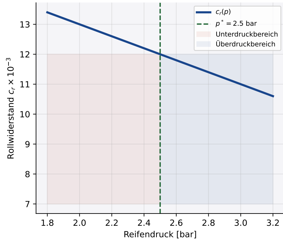
Rollwiderstand vs. Druck
