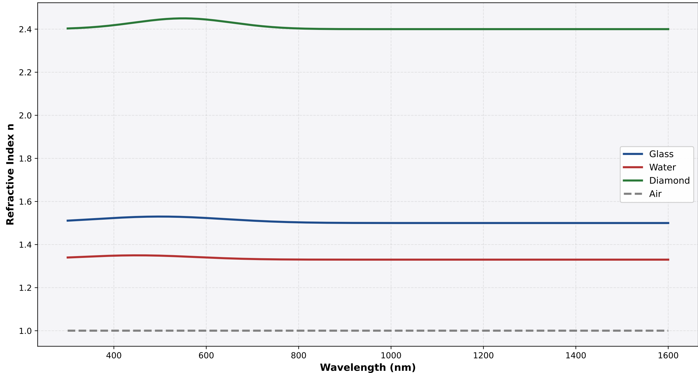
Refractive Index Variation Across Wavelengths
