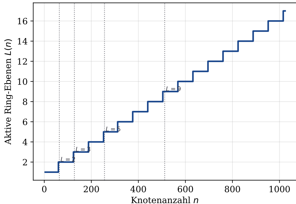
Stack-Tiefe L(n) = \lceil (n + \log_2 n) / 64 \rceil
