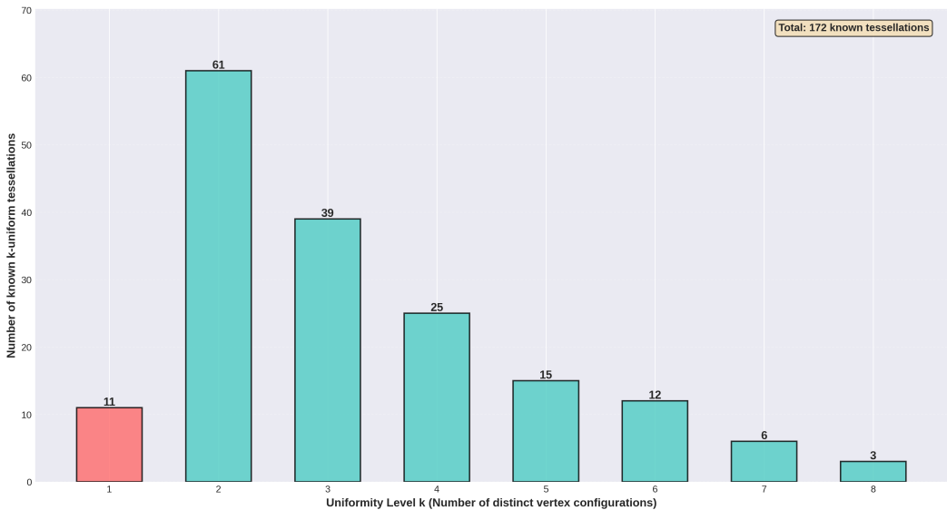
Enumeration of k -uniform Edge-to-Edge Tessellations of \square^2
