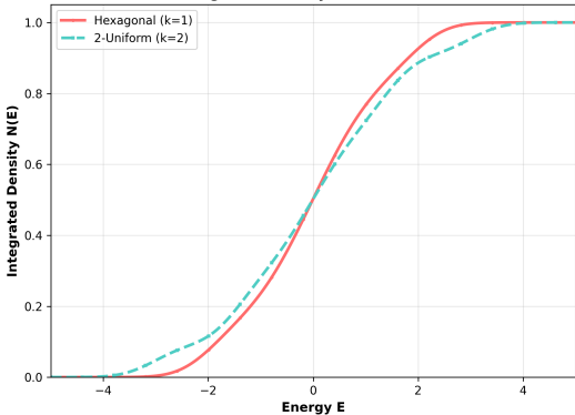
Integrated Density of States (IDS)
