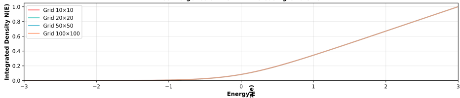
Convergence Rate Analysis
