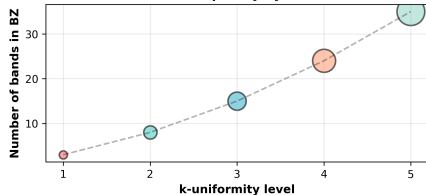
Band Complexity by k-level
