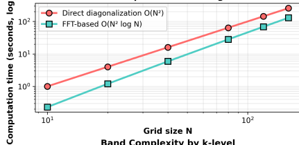
Band Complexity by k-level
