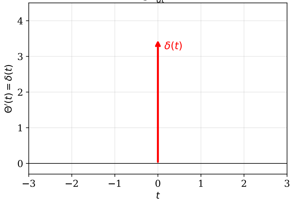
Ableitung: \frac{d}{dt}\Theta(t) = \delta(t)
