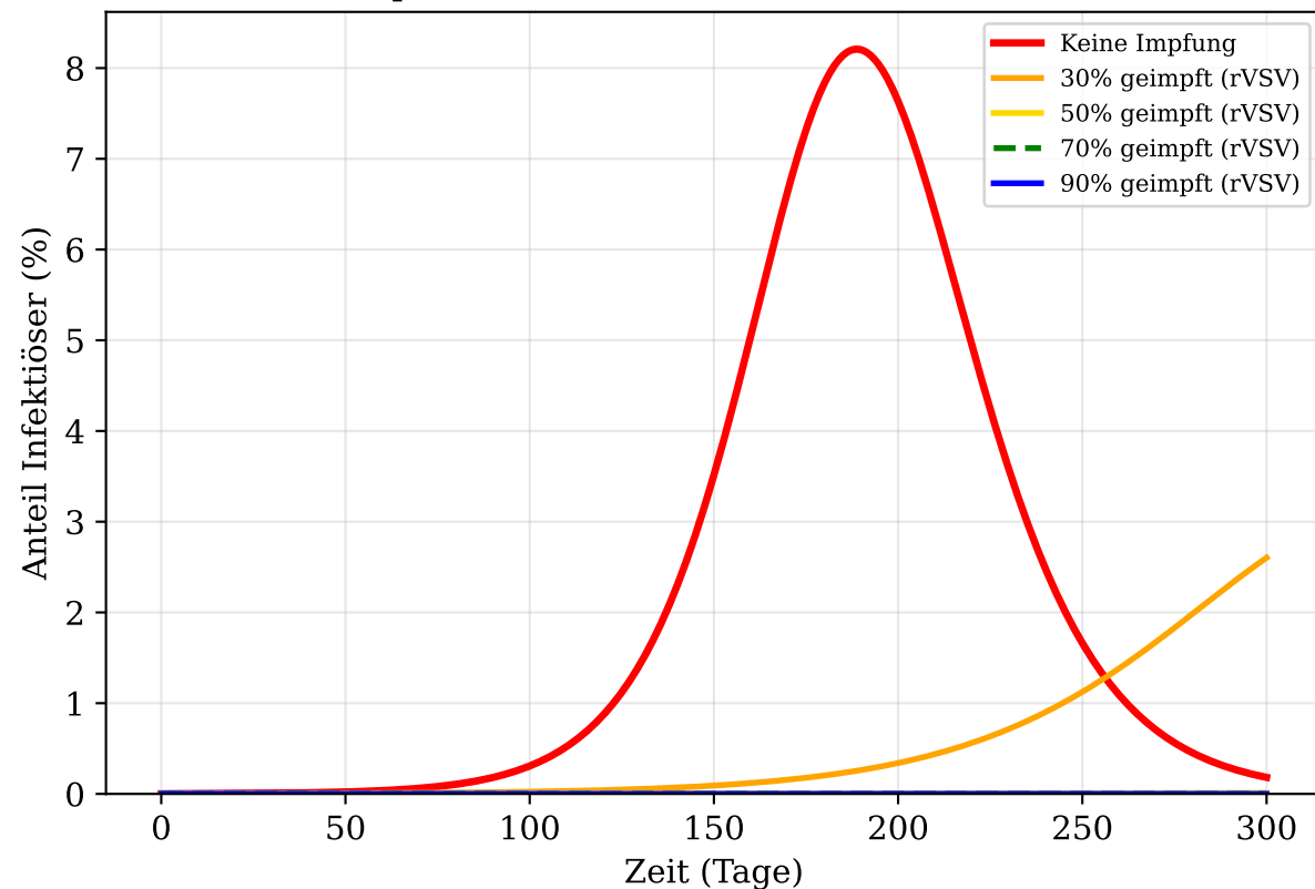
Impfszenarien (rVSV-ZEBOV, VE=97.6%)
