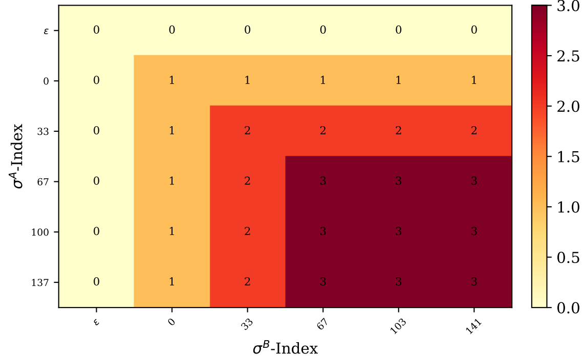
LCS-DP-Tabelle (LCS = 3)
