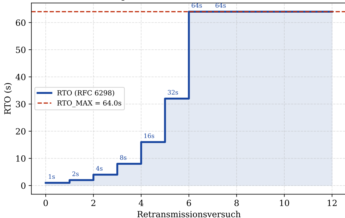
TCP Retransmission Timeout (Exponential Backoff, RFC 6298)
