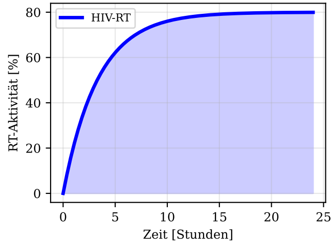
C: RT/RdRp-Kinetik
