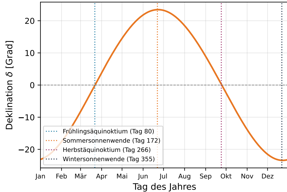
(a) Sonnendeklination \delta(t)
