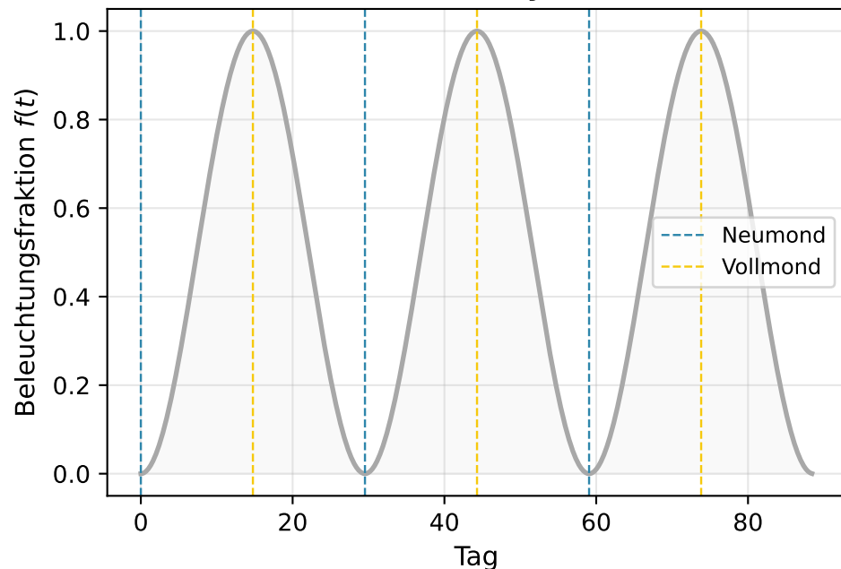
(a) Mondillumination (3 synodische Monate)
