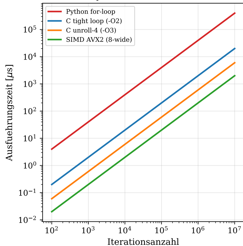
Loop-Performance: Python vs. C vs. SIMD
