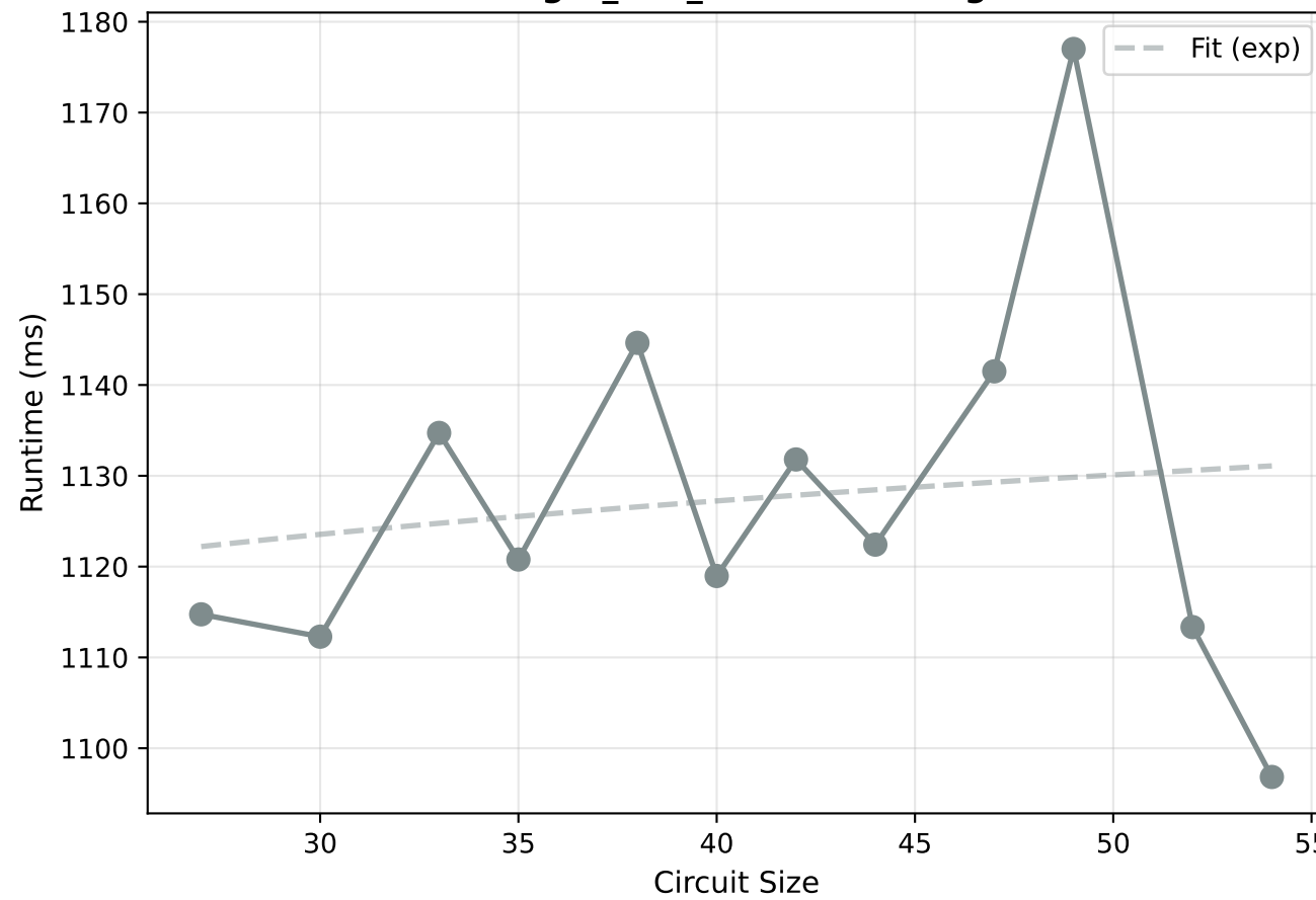
Target_and_random Scaling
