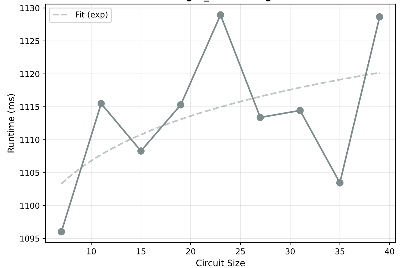
Target_and Scaling
