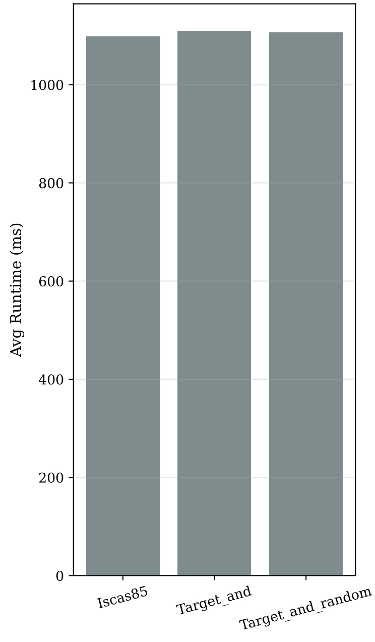
Average Runtime
