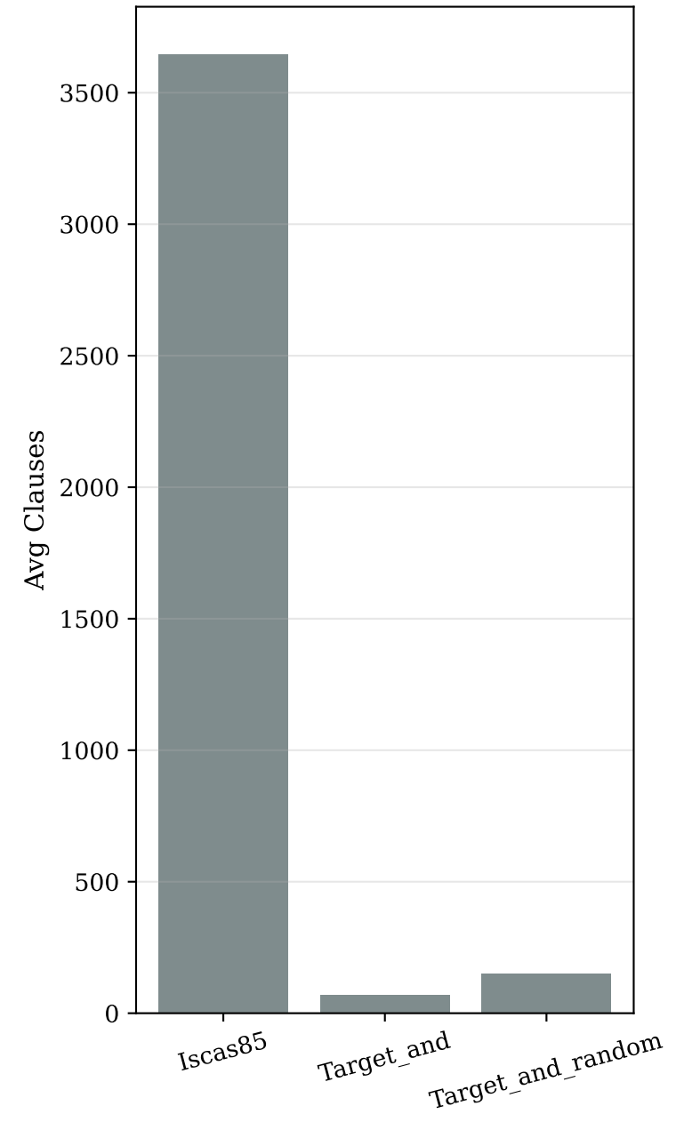
Average Clauses
