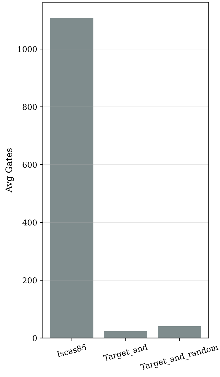
Average Gates
