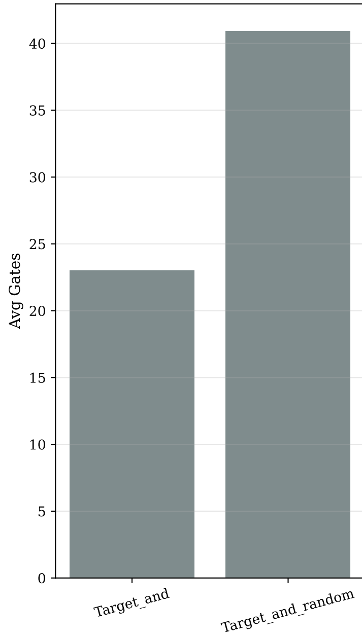
Average Gates
