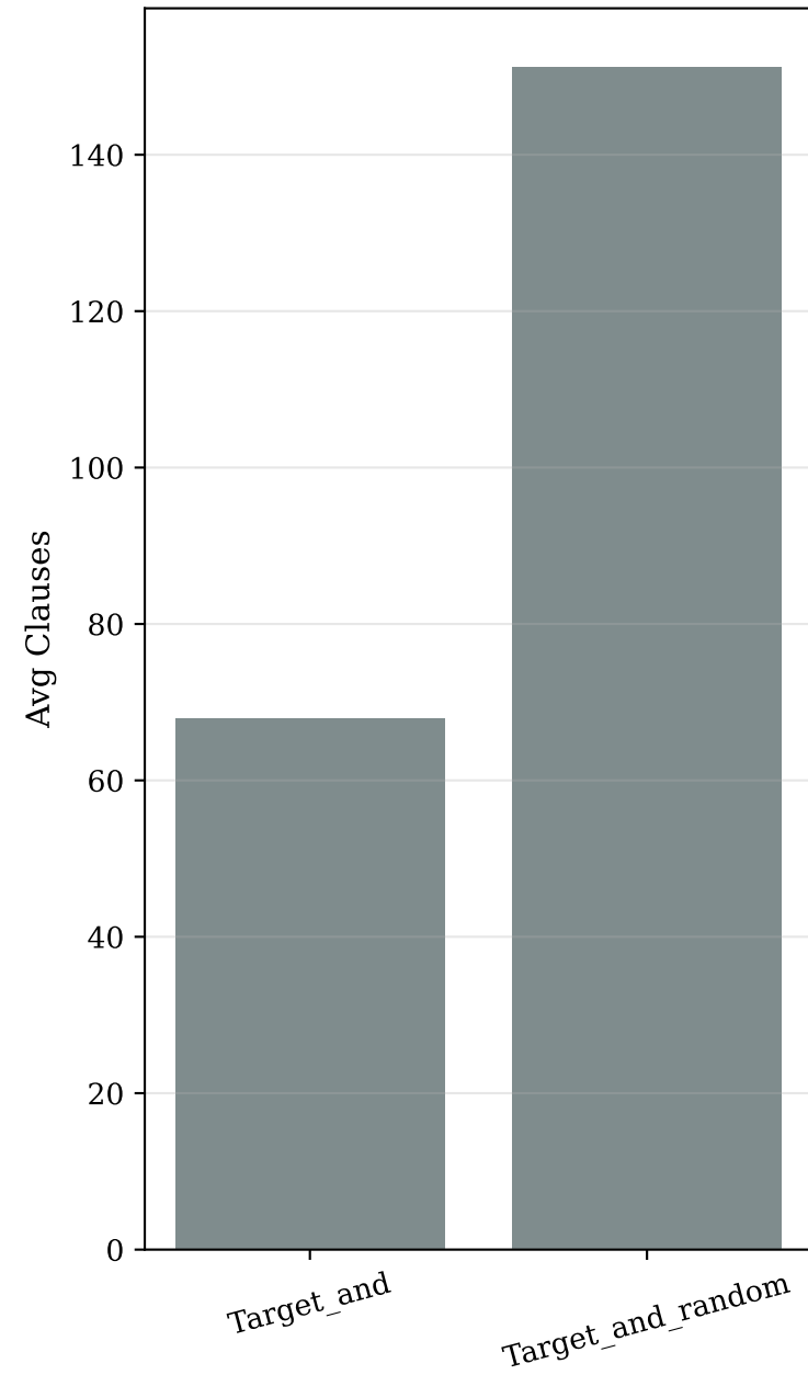
Average Clauses
