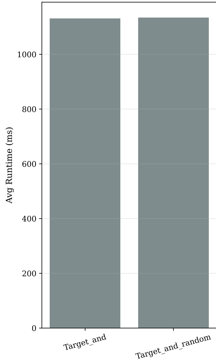
Average Runtime
