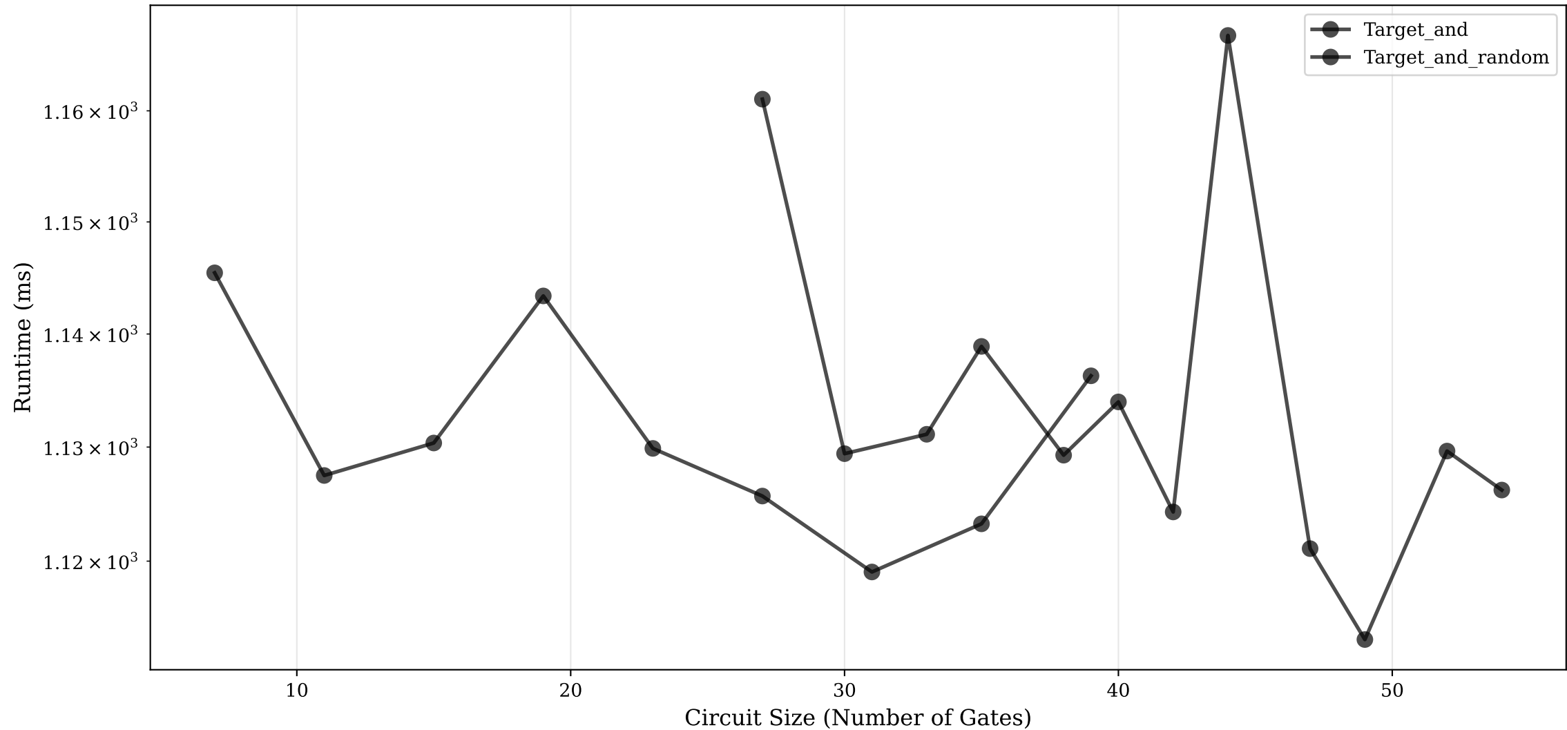
Subgraph-SAT-Solver: Runtime vs. Circuit Size
