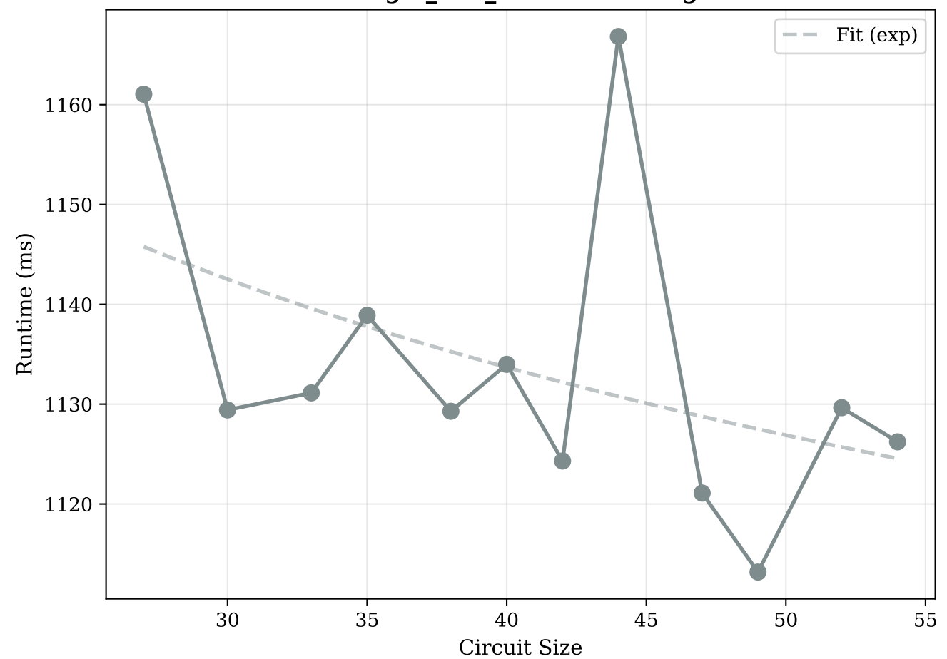
Target_and_random Scaling
