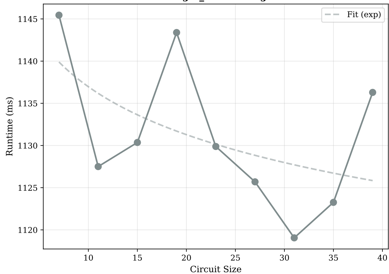
Target_and Scaling
