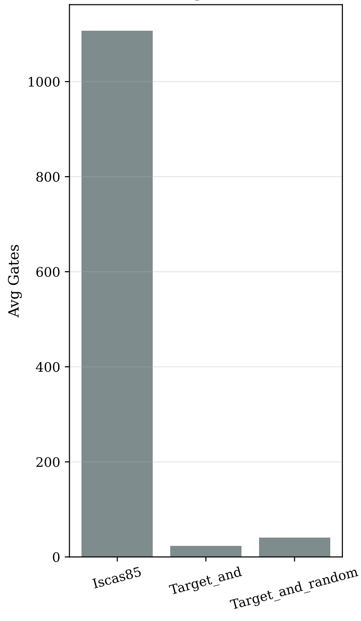
Average Gates
