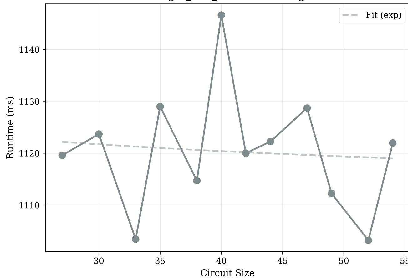
Target_and_random Scaling
