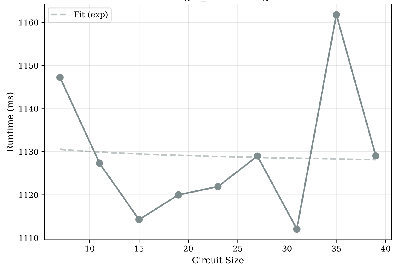
Target_and Scaling
