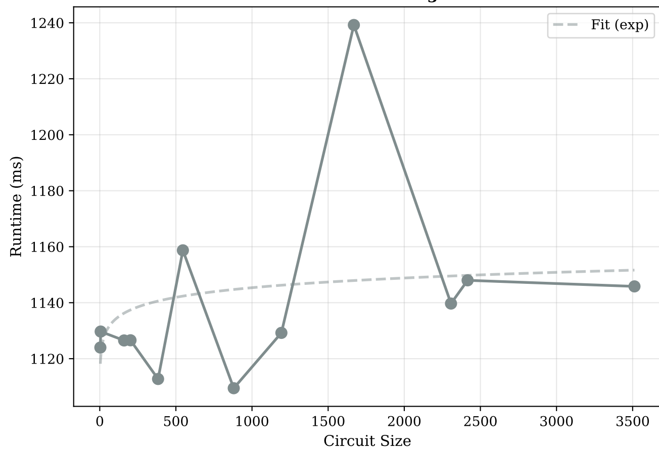
Target_and_random Scaling
