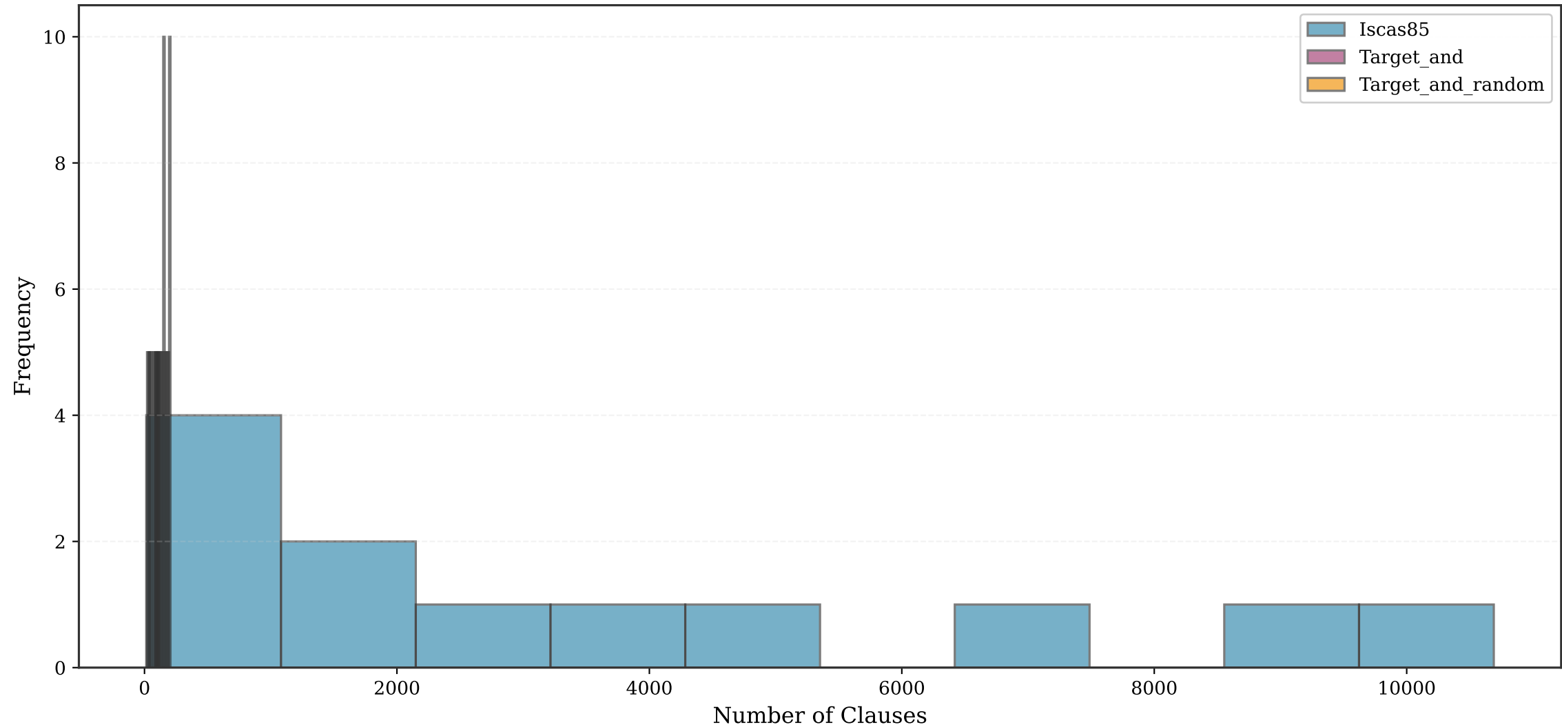
Subgraph-SAT-Solver: CNF Clause Distribution
