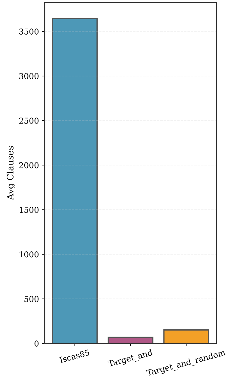
Average Clauses
