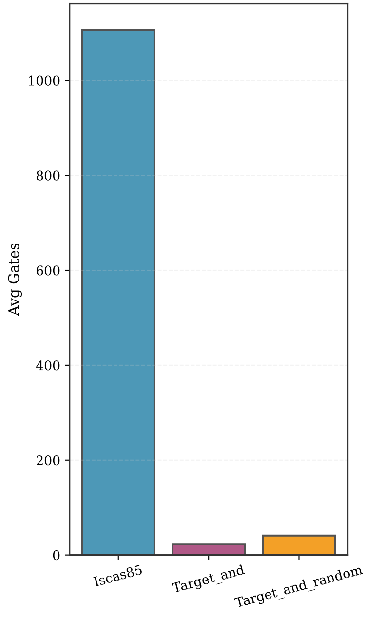
Average Gates
