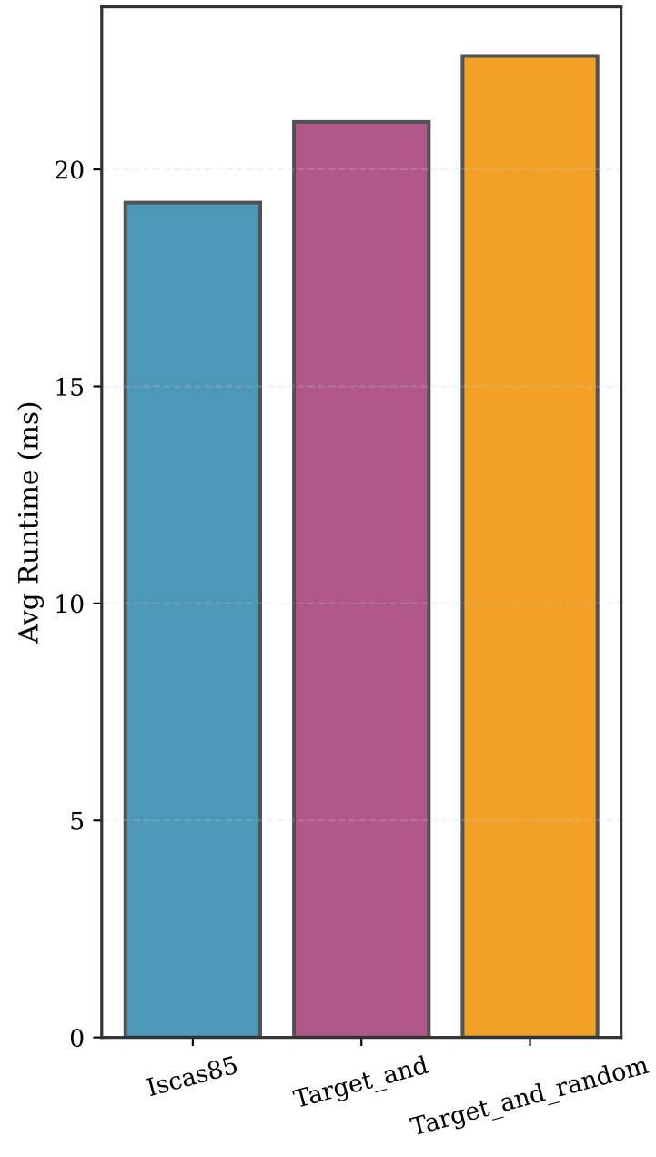
Average Runtime
