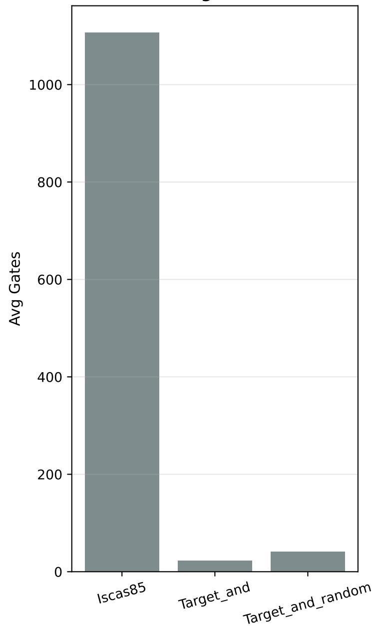
Average Gates
