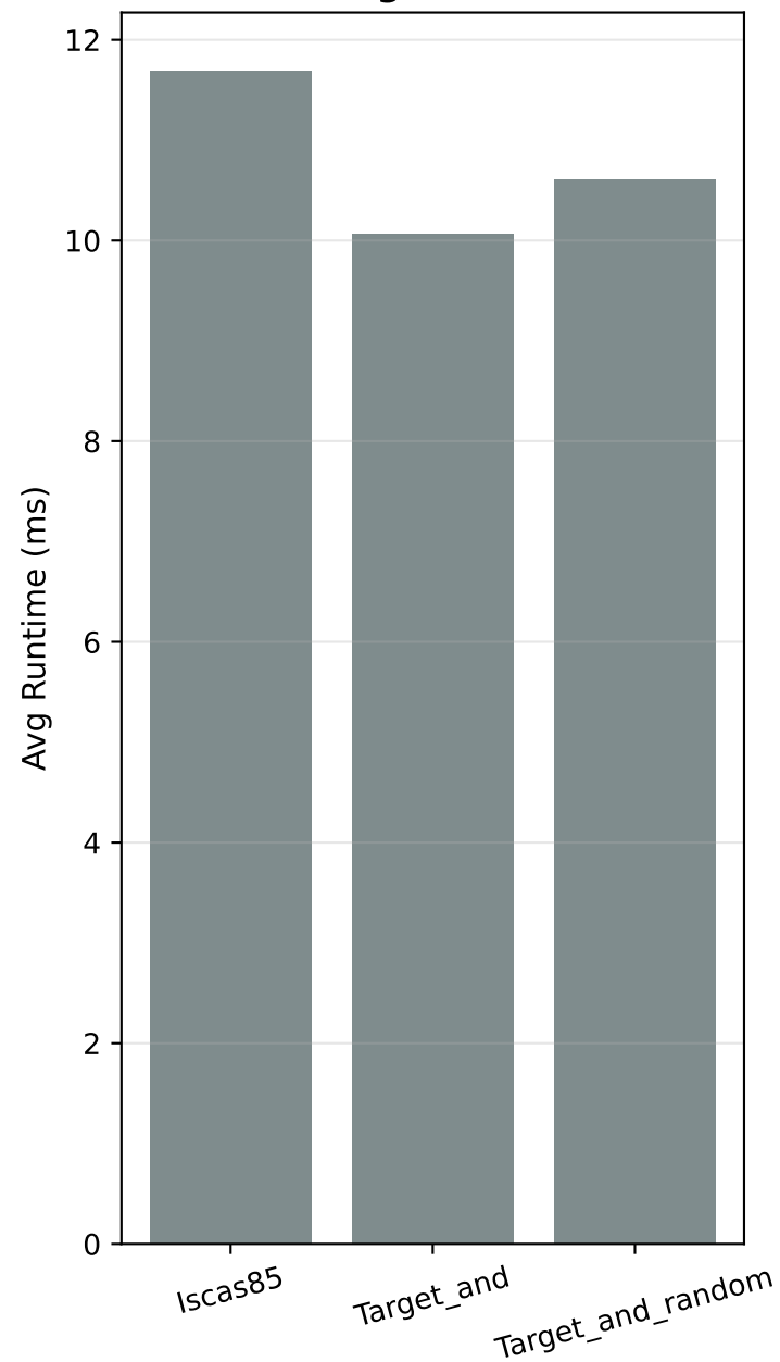
Average Runtime
