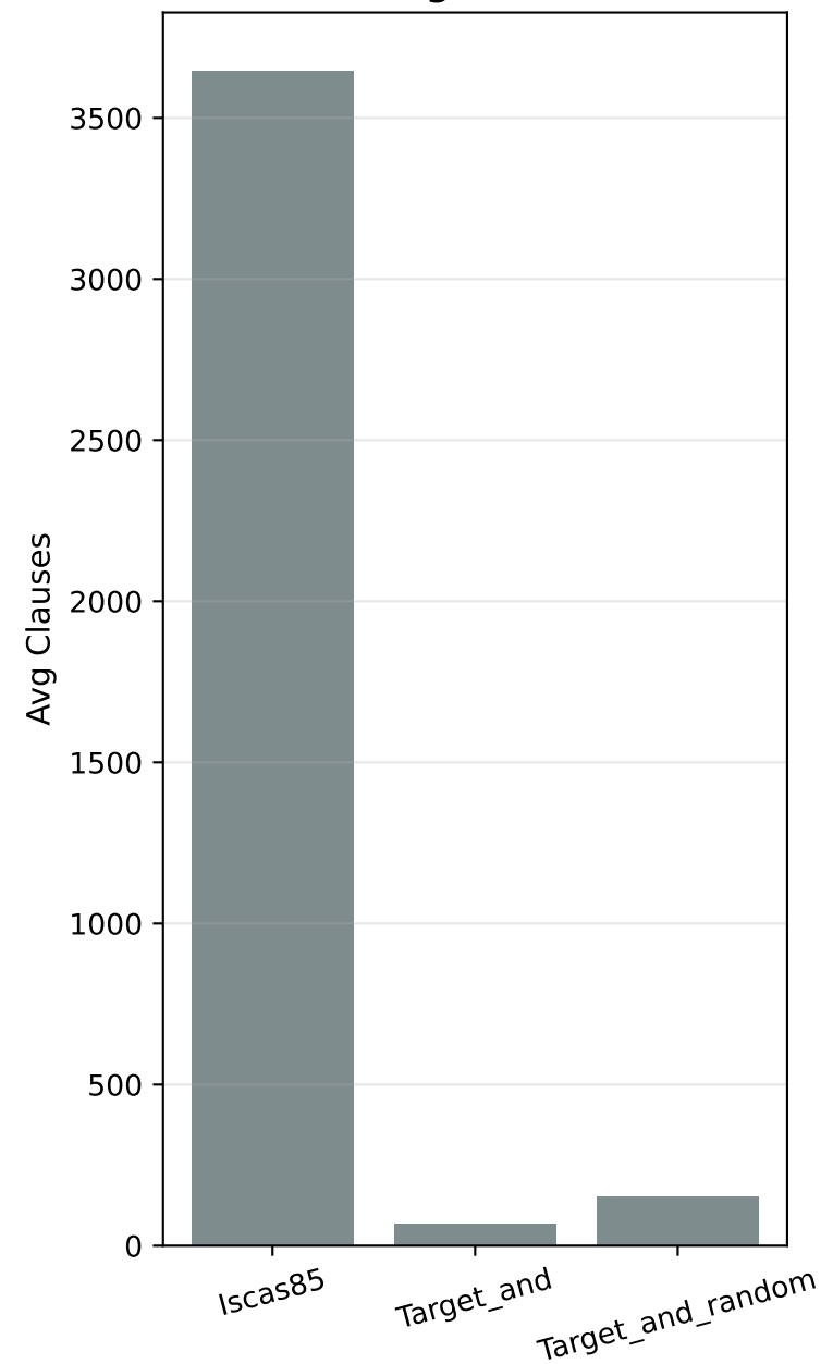
Average Clauses
