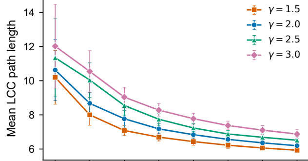
a Paths by tail exponent ( n = 300 )
