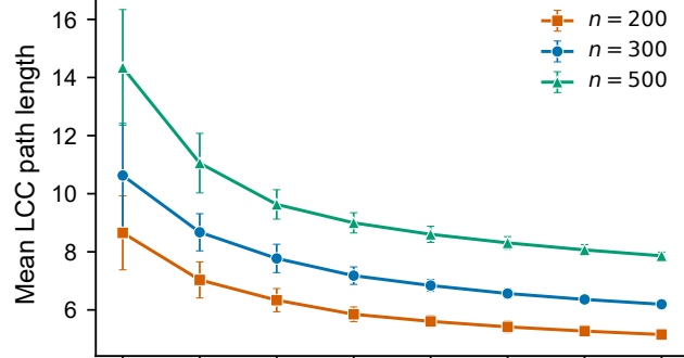
b Paths by system size ( \gamma = 2 )
