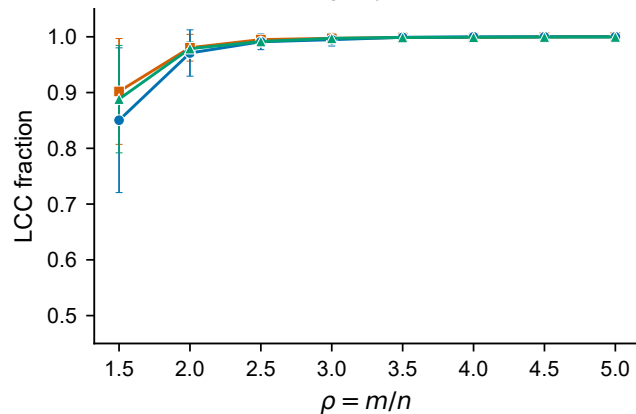
d Component coverage by n
