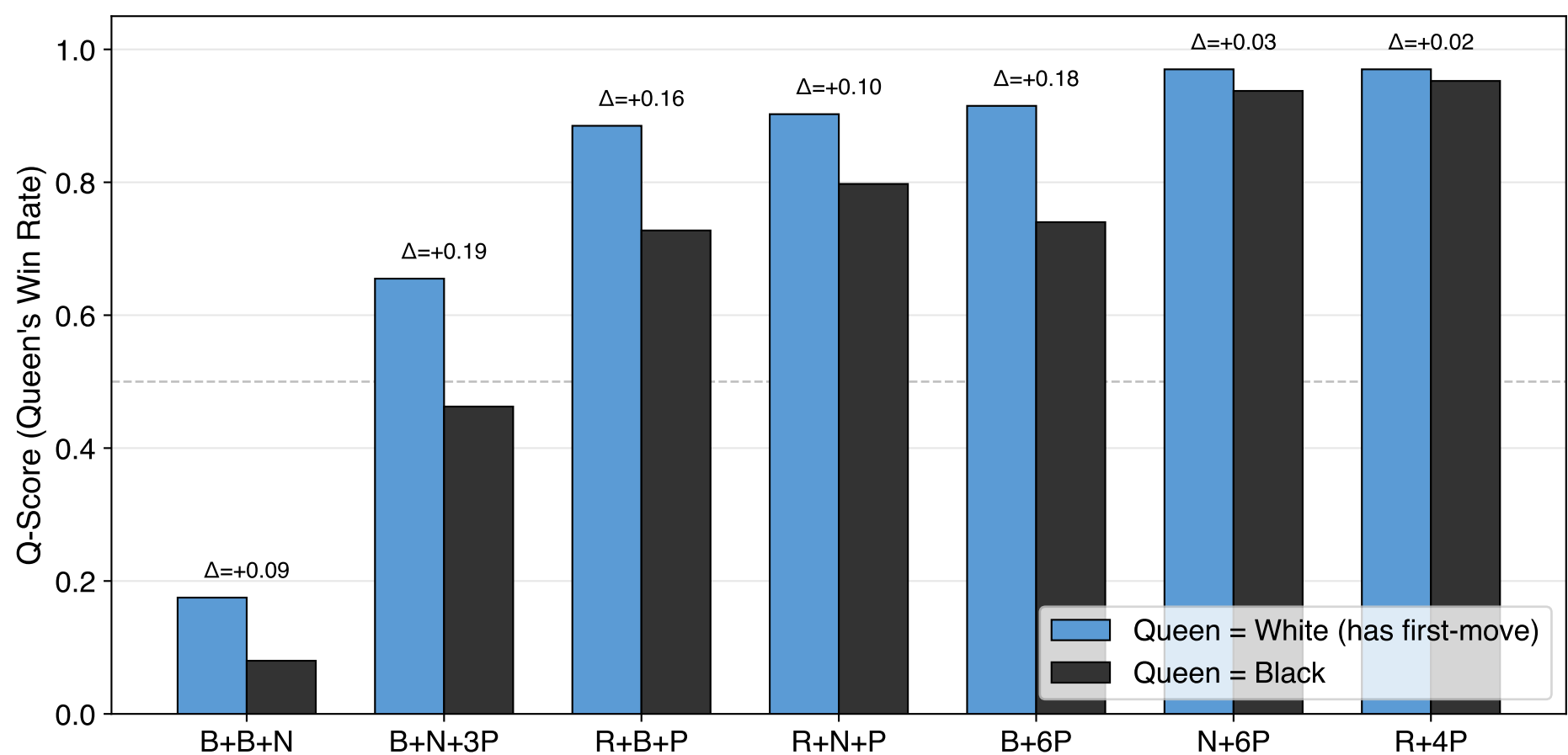
Figure 5: Color Asymmetry (Lc0)
